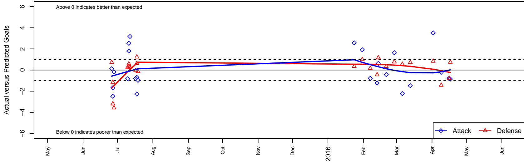
HSC Arsenal B99 Dots are actual minus expected GF (blue circles) and GA (red triangles). Blue line is smoothed change in attack strength. Red is smoothed change in defense strength.
